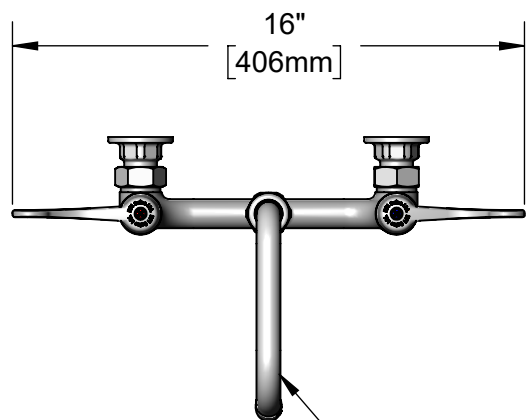
SIF-SN06 6" Swing Nozzle w/ Laminar Flow Outlet Device
