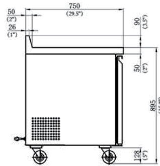
SECTION VIEW
